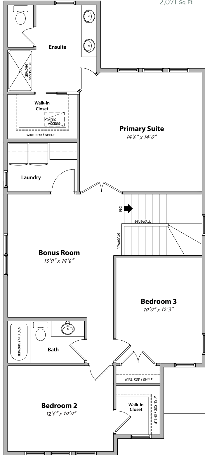
Second Level 1,114 sq.ft.
