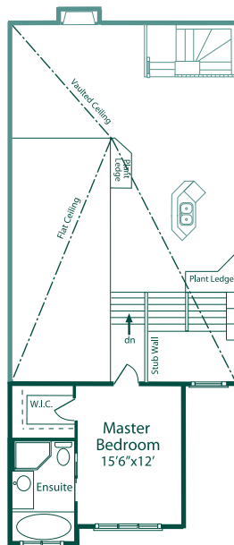
Upper Level 356 Sq. Ft.
