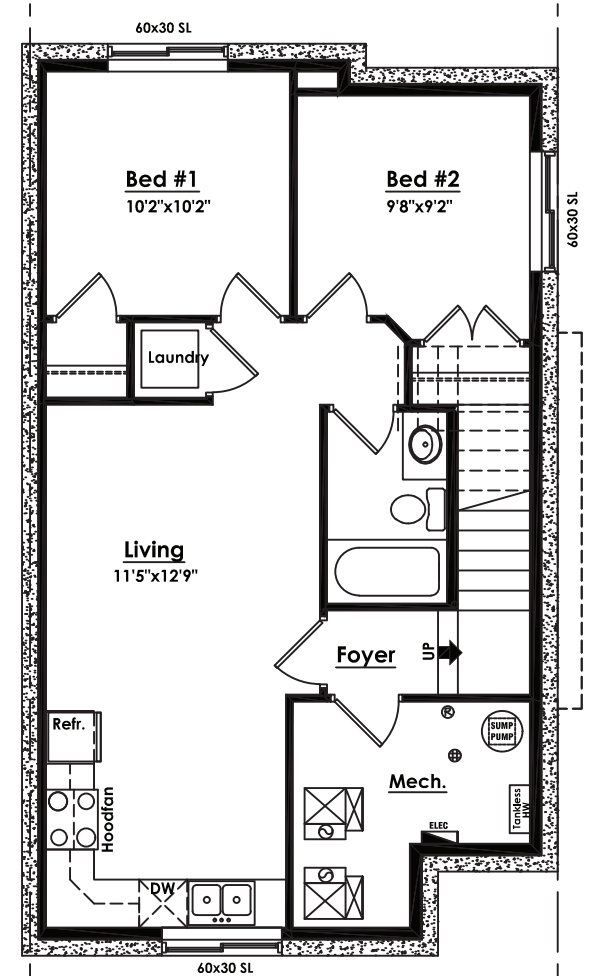
(Optional) Secondary Suite 693 sq. ft.
